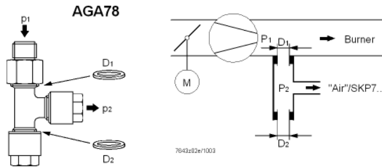
Figure 11 AGA78 Operation.
