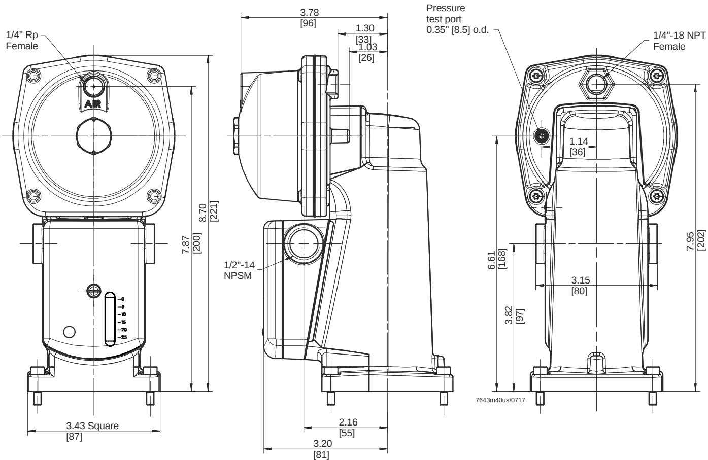
Figure 15. SKP25.0xxUx dimensions
