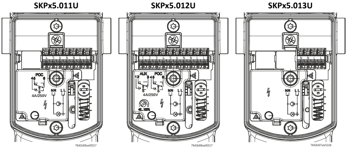
Figure 13. Terminal designations
