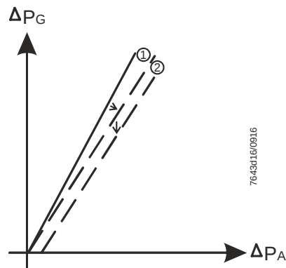
Figure 10. SKP75.xxxUx Adjustments
