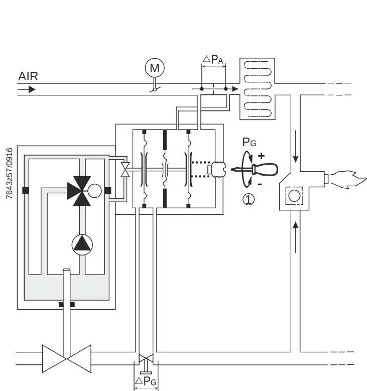
Figure 3. SKP55.xxxUx operation
