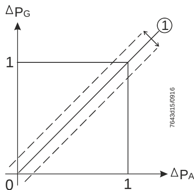
Figure 9. SKP55.xxxUx Adjustments
