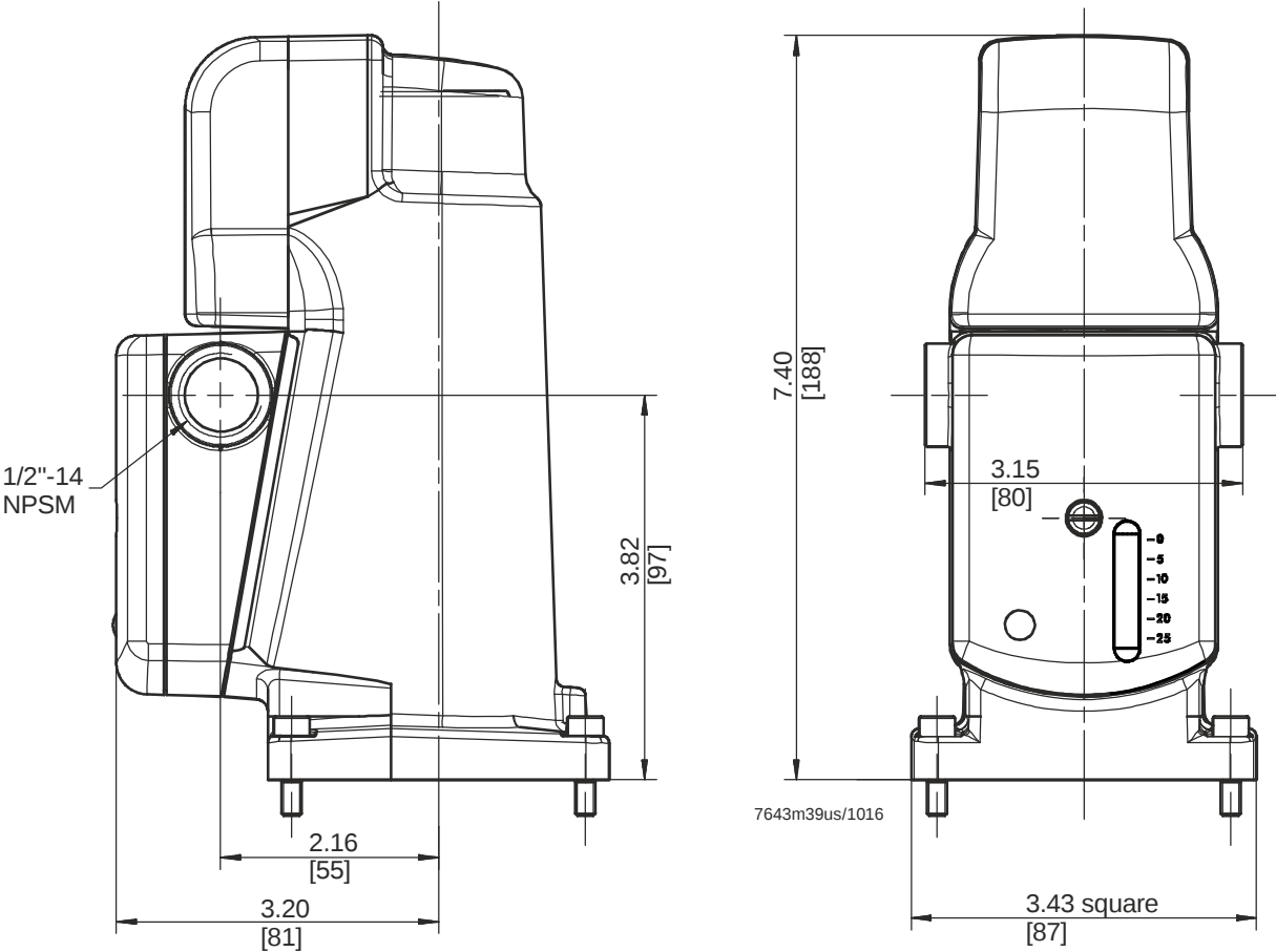
Figure 14. SKP15.xxxUx dimensions
