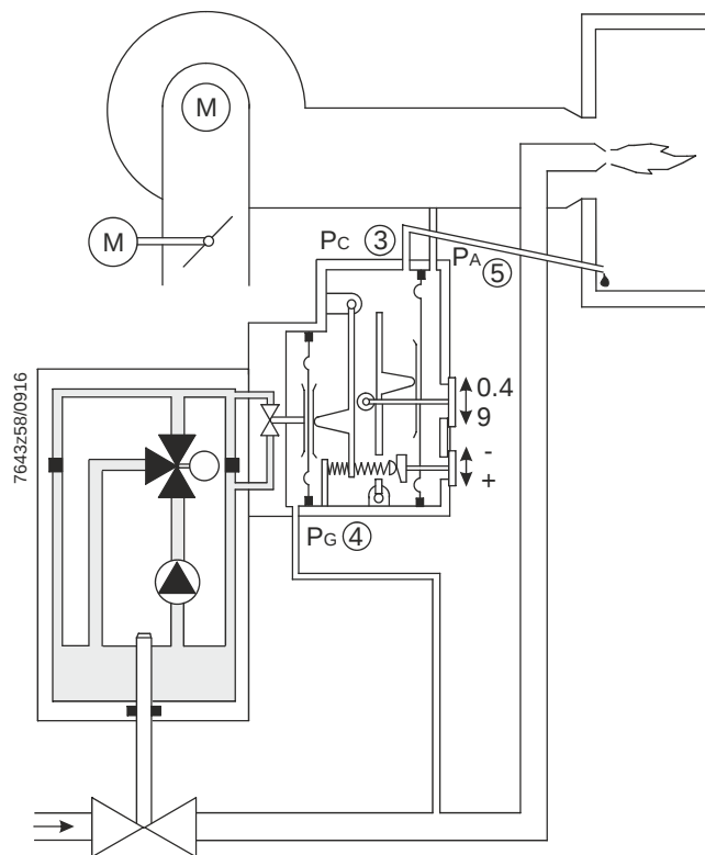
Figure 4. SKP75.xxxUx operation
