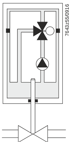
Figure 1. SKP15.xxxUx operation
