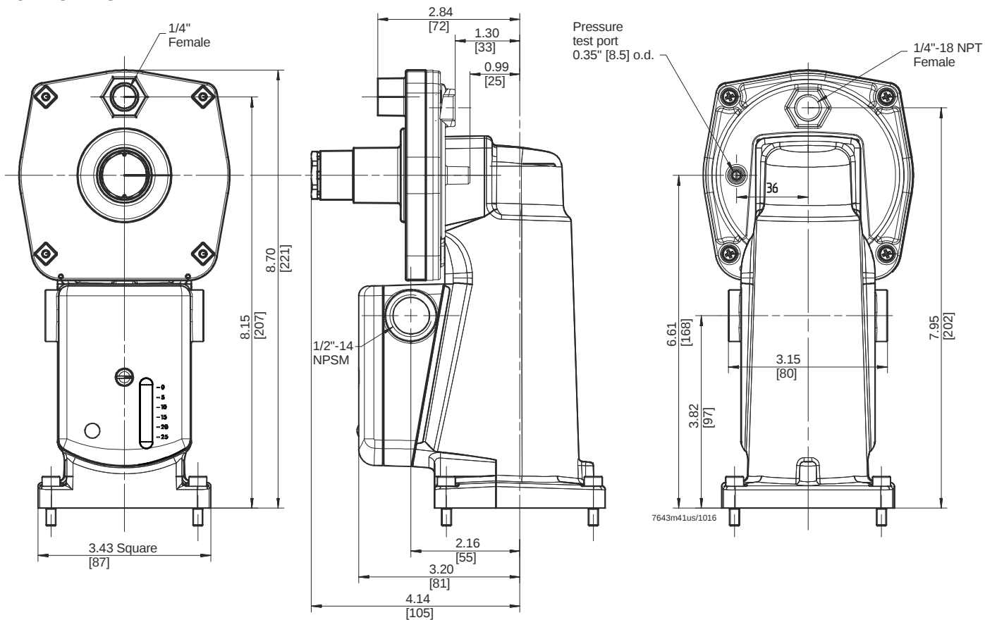
Figure 16. SKP25.4xxUx dimensions
