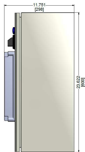
Side (NEMA 12 with cover)
