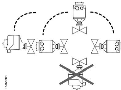
Figure 1. Acceptable Mounting Positions.
