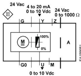
Figure 3. Wiring Diagram.
