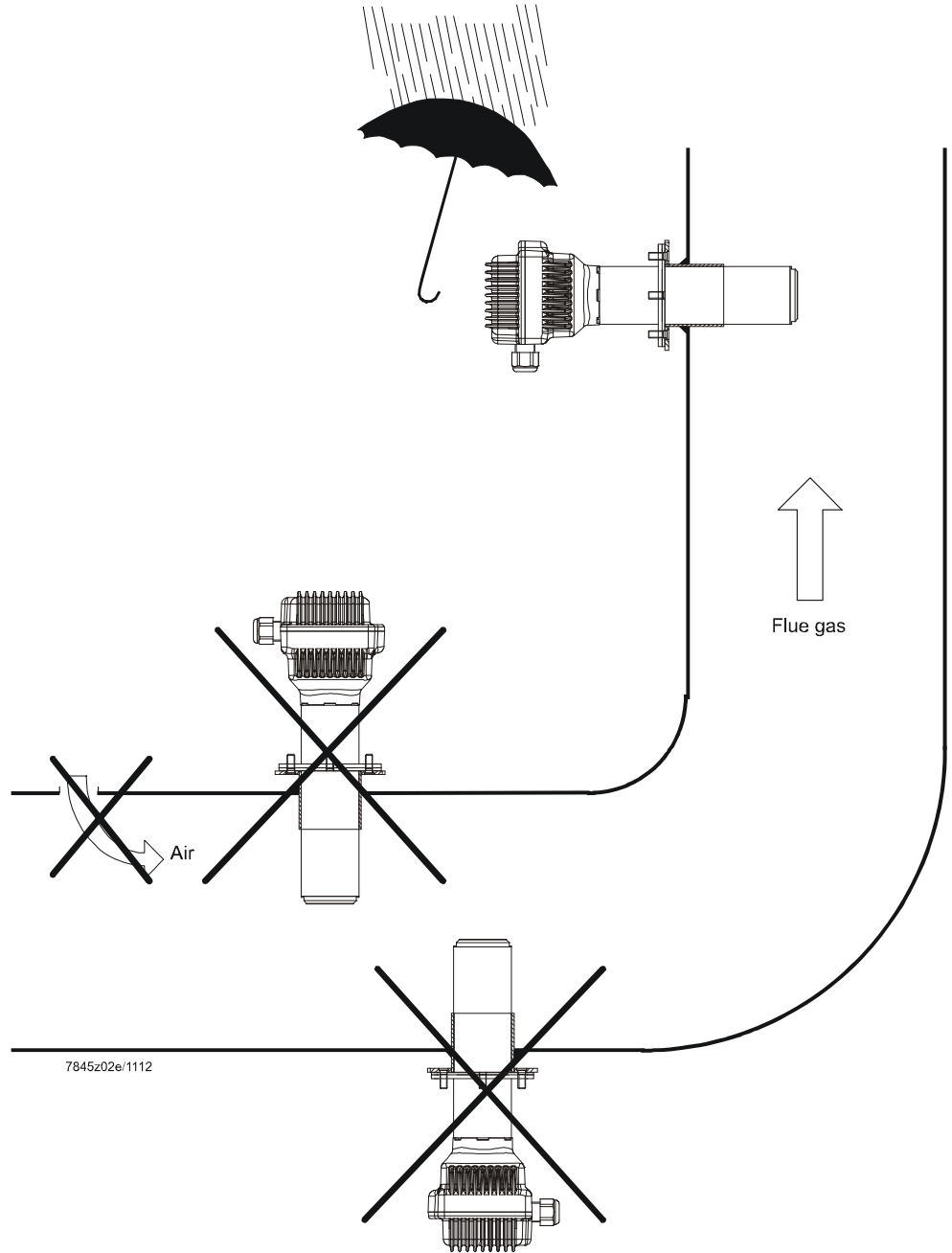
Figure 8: Mounting position of QGO21
