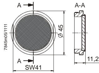
Figure 14: Dimension AGO7428700120
