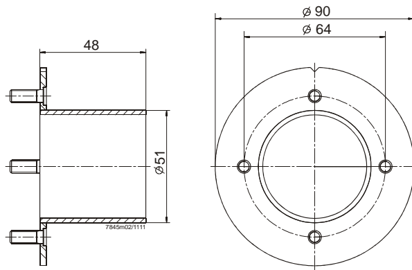
Figure 13: Dimension AGO21...
