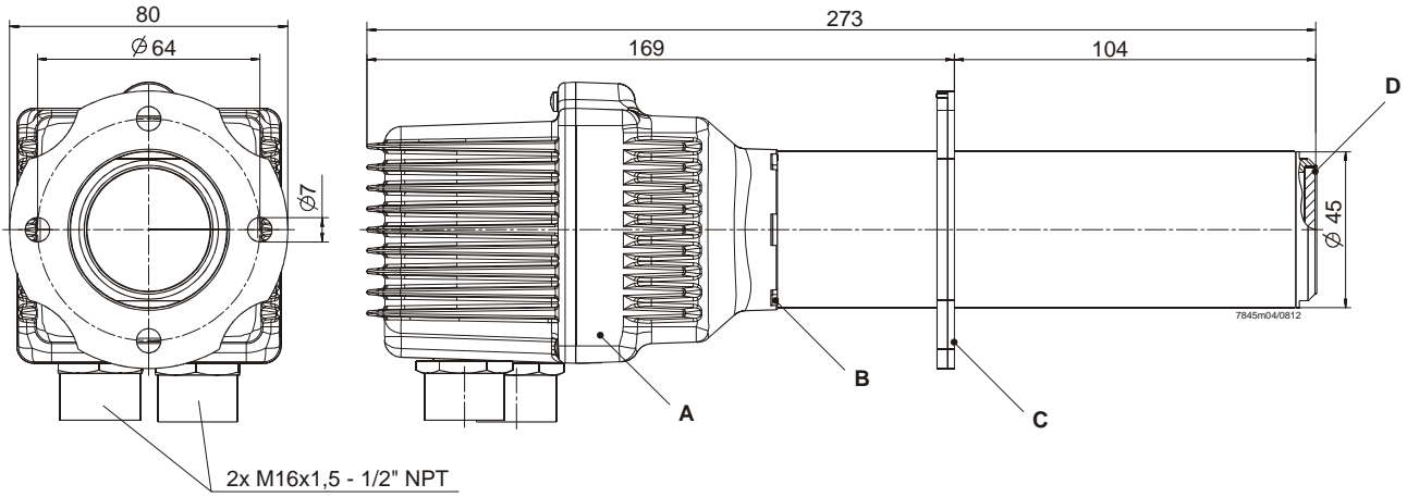
Figure 11: Dimension QGO21.000D27
