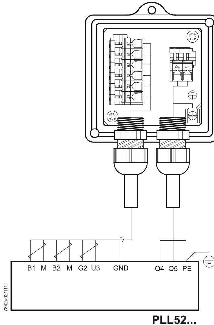
Figure 9: Connection QGO21
