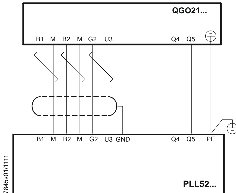
Figure 10: Connection diagram
