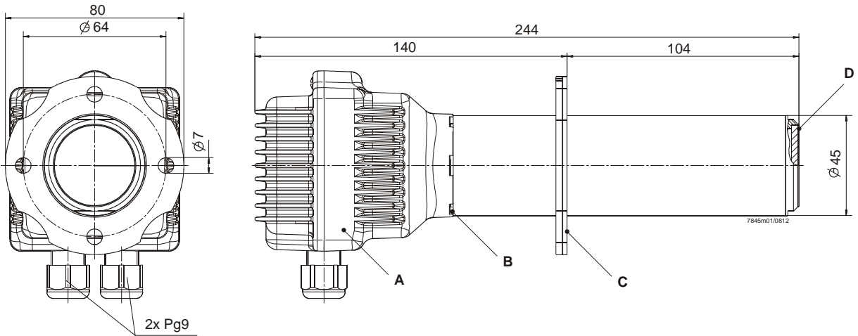
Figure 12: Dimension QGO21.000D17
